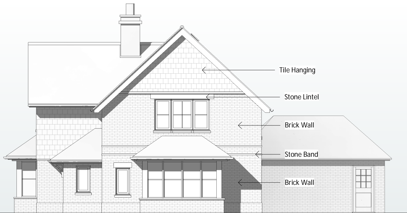
PLOT 18 Side - South West Elevation
